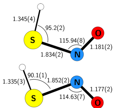
Figure 2. Structure of cis - (top) and trans -HSNO (bottom) determined in this study (semi-experimental equilibrium structure, see Table S1). Bond lengths are in Å and angles in degrees.
