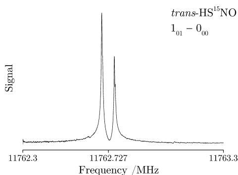
Figure 1. FTMW spectrum of the two Doppler components of the 1_{01}-0_{00} transition of trans -HS 15 NO (integration time: ~1 min).
