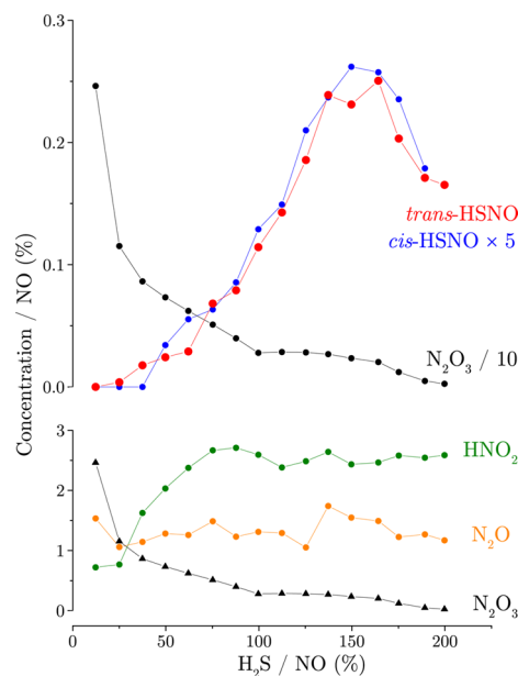
Figure 3. Change in the concentration of several NO containing molecules upon addition of H 2 S to the NO gas stream.
